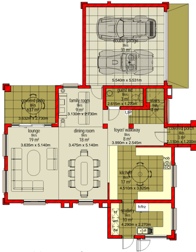
1 02 ground 1 : 100
