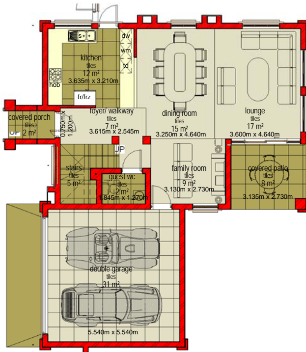
1 02 ground 1 : 100
